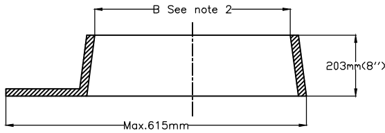
Tapered guide frame
