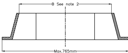
Tapered guide frame
