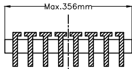
Self-lock grate
