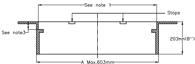
Adjustable frame
